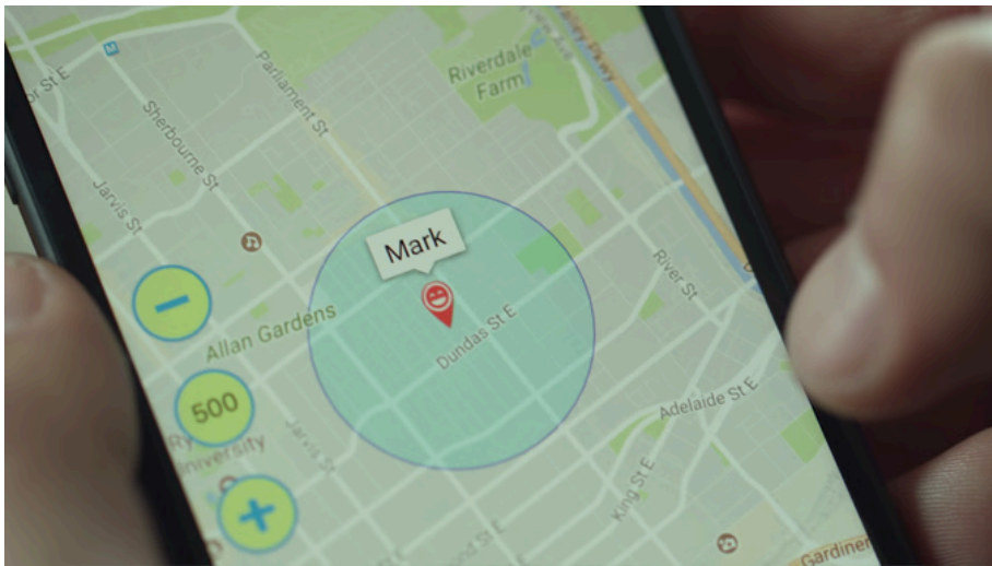
Geo-Fence
